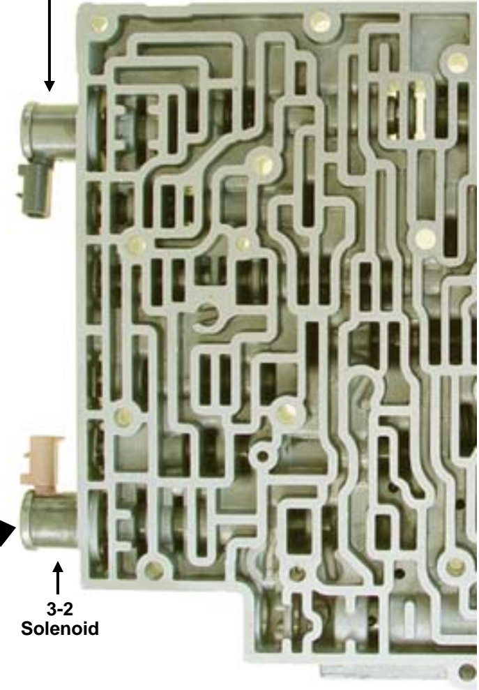
PWM Solenoid
